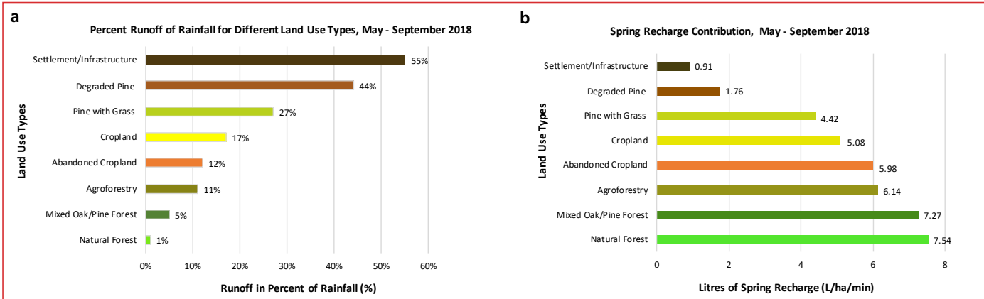
Figure 8a) Percent runoff of rainfall for different land use types. The calculation assumed total of 957 mm from daily local rainfall records (between May and September 2018); 8b) Spring Recharge Contribution (Liters/ha/minute) are compared for different land use types 15 .
